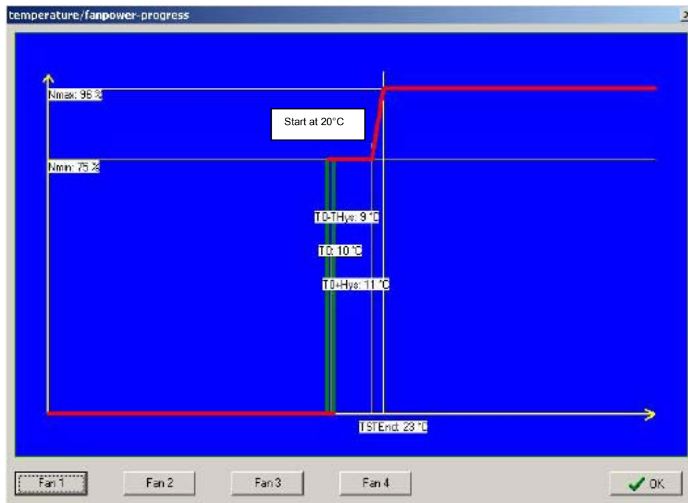
fan control characteristic (factory setting)
